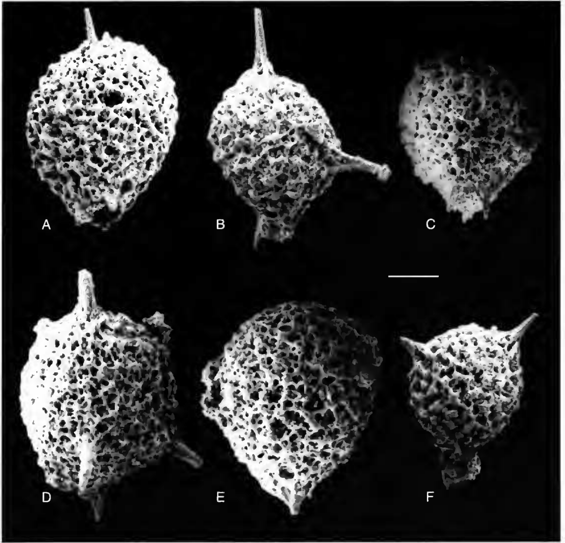
FIG. 9. — Glomeropyle boreale Bragin, n. sp.; A, holotype; B-F, paratypes. Northeastern Siberia, Omolon Massif, Dzugadzak River, Middle Triassic, Ladinian, Unit 10. Scale bar: 100 \mu m.
